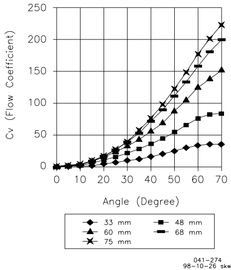
Cv for Standard Flo-Tech Units
